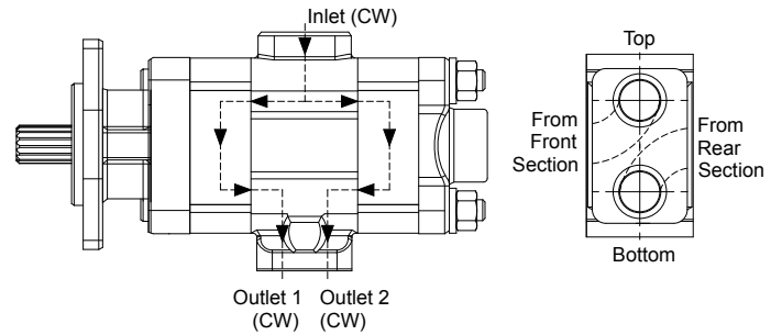
Tandem Unit Flow Diagram (CW Rotation) 1 Inlet, 2 Outlet Style Bearing carrier shown
