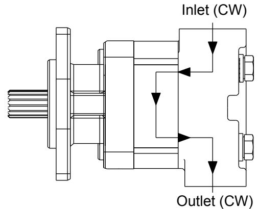
Single Unit Flow Diagram (CW Rotation)
