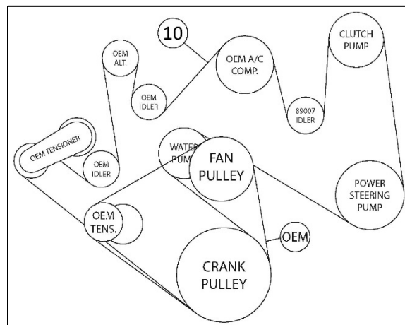
Belt Routing (10)
