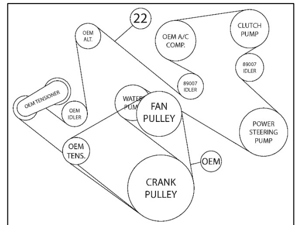
Belt Routing (22)
