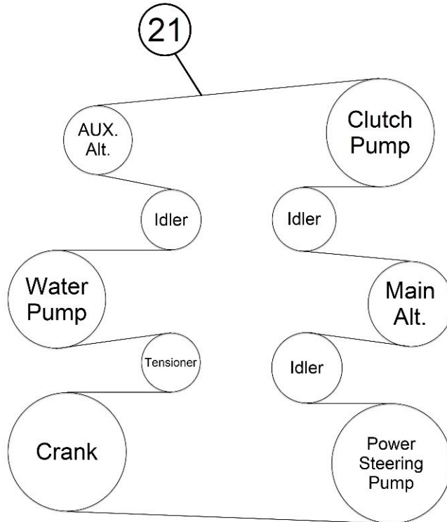
Belt Routing (21)
