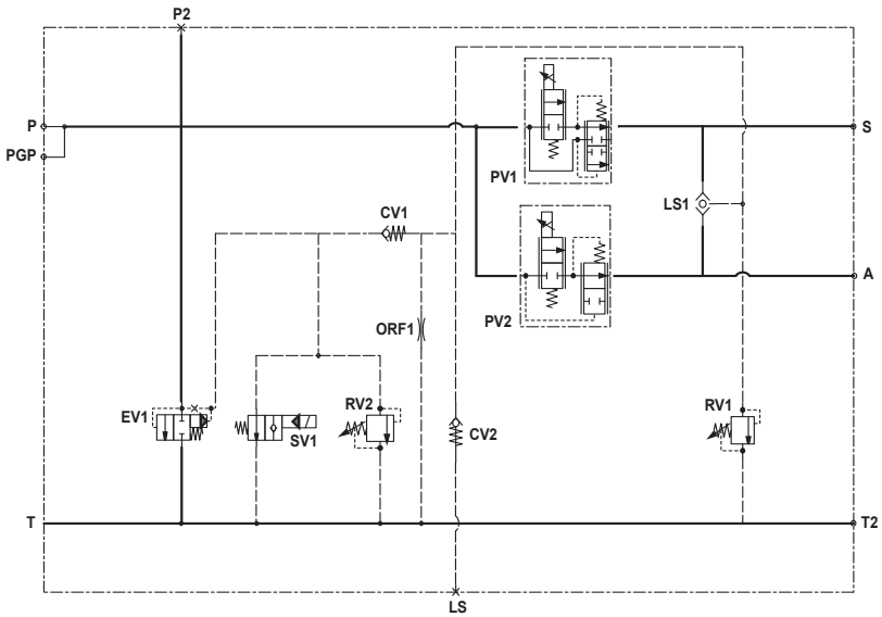
HF42407-07 VALVES
