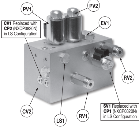
HF42407-07 VALVES
