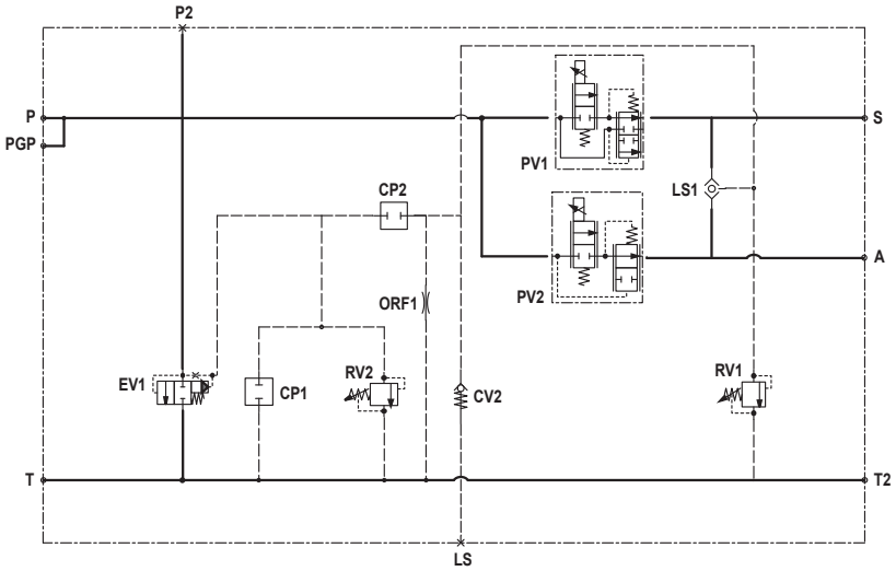
HF42407-07 VALVES
