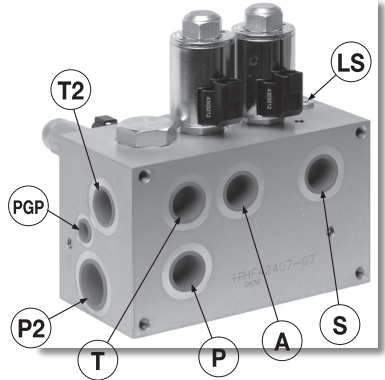
HF42407-07 PORTS
