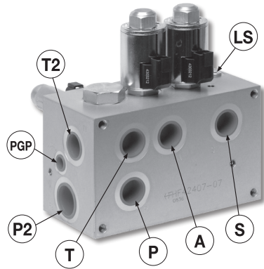
HF42407-07 PORTS
