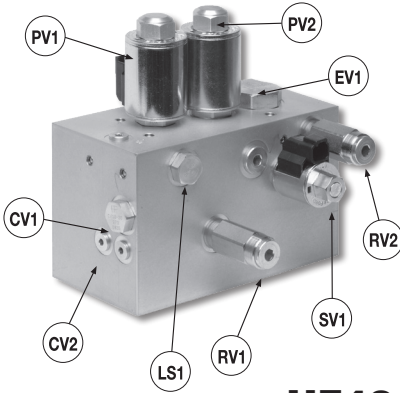
HF42407-07 VALVES
