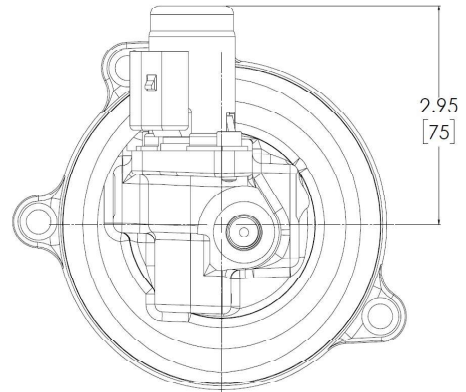
New solenoid valve and rear cover Units built on or after 2/21/2025
