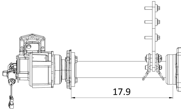
New XSMC-A40XX-X3**XX Housing Length
