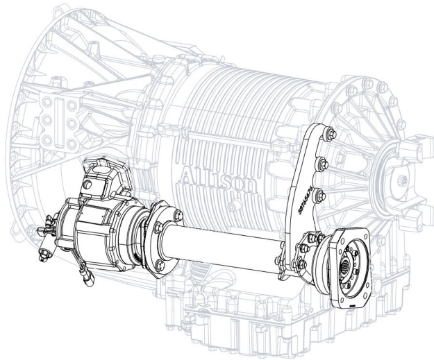
XSMC with new Clamping Style Bracket
