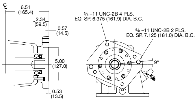
SAE "C" 2- & 4-Bolt 1 1/4" -14 Spline ("E" Option)
