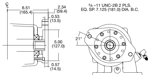
SAE "C" 2-Bolt 1 1/4" -14 Spline ("Y" Option)
