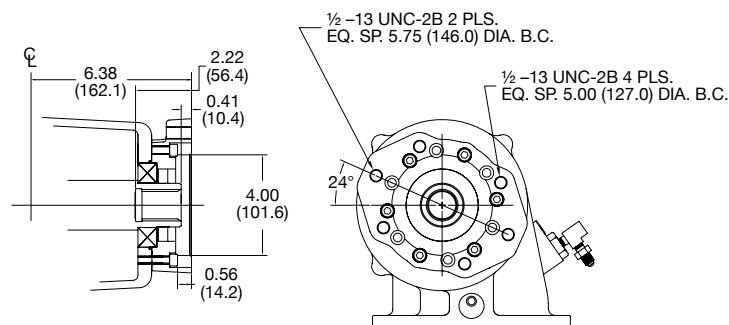
SAE "B" 2- & 4-Bolt 1 1/4" -14 Spline ("Z" Option)
