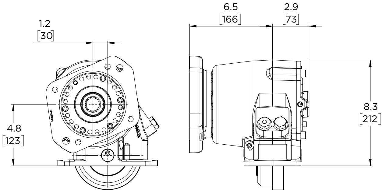
SAE C 2- & 4-Bolt 1 1/4" -14T Spline Output ("E" Option)
