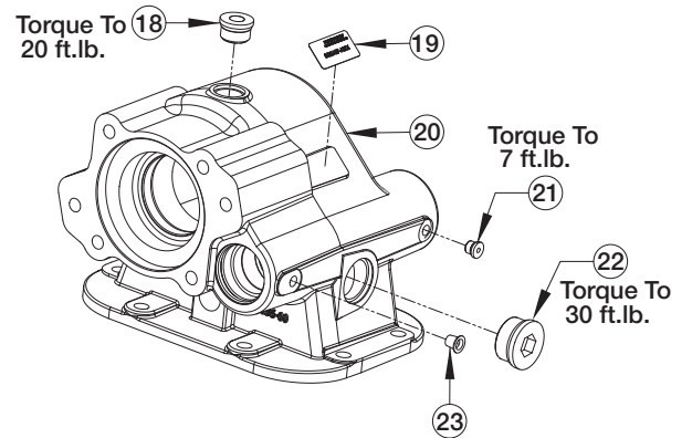
DETAIL C: PTO HOUSING
