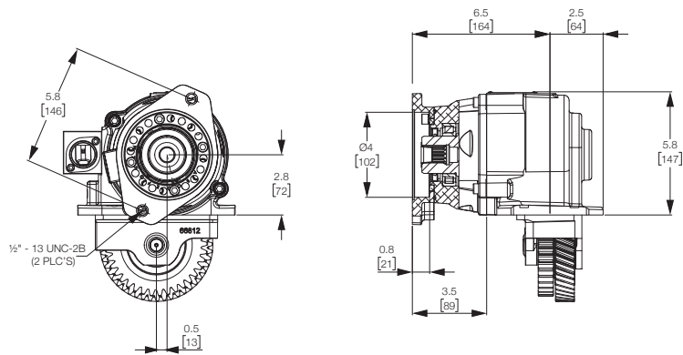
BS OUTPUT — SAE “B” 2-Bolt, 7/8" -13T SPLINE
