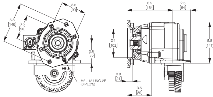
BB OUTPUT — SAE “B” 2- & 4-BOLT, 7/8" -13T SPLINE PB OUTPUT — SAE “B” 2- & 4 BOLT, 1" -15T SPLINE
