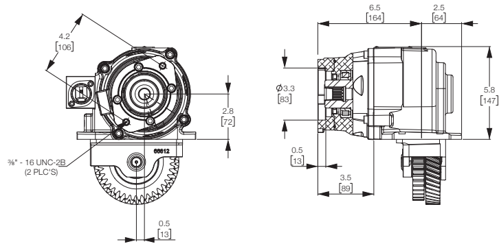
TA OUTPUT — SAE “A” 2-Bolt, 3/4" -11T SPLINE BA OUTPUT — SAE “A” 2-Bolt, 7/8" -13T SPLINE
