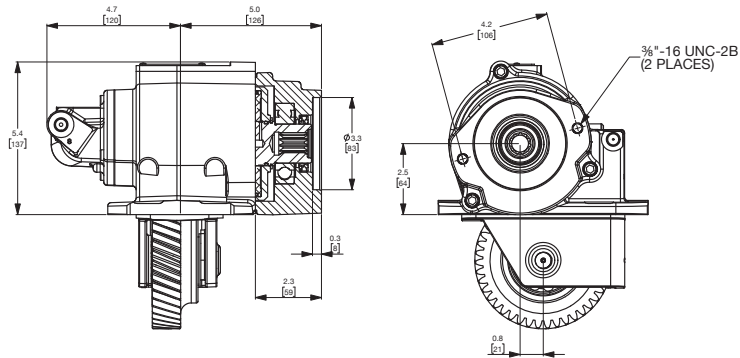
“TA” OUTPUT — SAE \frac{3}{4} " -11T, SAE “A” 2-Bolt
