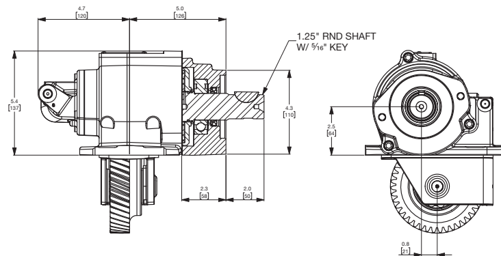
“1X” Output -1 \frac{1}{4} " Round Keyed Shaft
