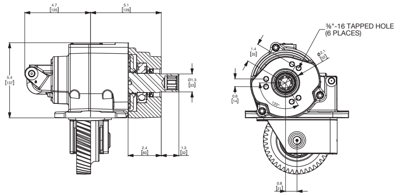
“UU” OUTPUT — UNI 222 Mount 3-Bolt Flange
