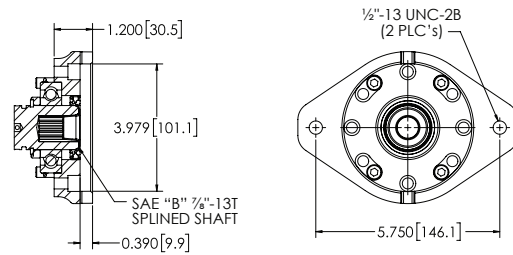
“S” Output – SAE “B” 2-Bolt Flange
