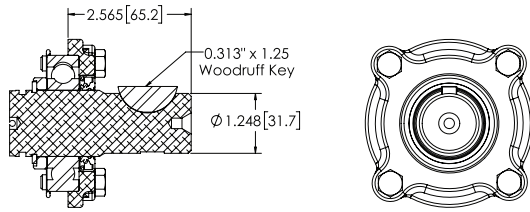
“B” Output – 1.250" Rnd Shaft w/ \frac{5}{16} " Key
