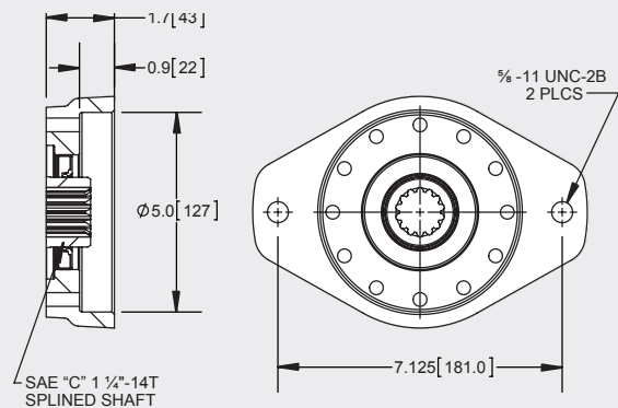
"Y" OUTPUT - SAE "C" 2-BOLT
