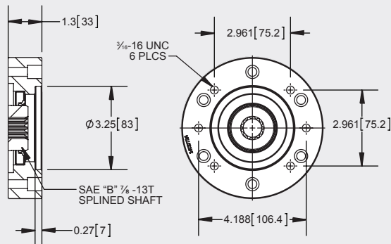
"Q" OUTPUT - SAE "A" 2- /4-BOLT FLANGE SAE "B" \frac{3}{4} "-13T SHAFT
