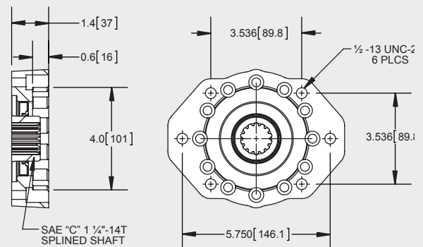
"Z" OUTPUT - SAE "B" 2- /4-BOLT FLANGE SAE "C" 1 \frac{1}{4} "-14T SHAFT
