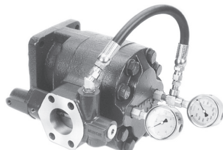
Pumps which are designed to easily accommodate vacuum and pressure gauges save maintenance time and provide greater accuracy. The special rear test ports shown in this view of the Muncie Power-Pro may be used for monitoring performance. The birotational four-port pumps (K & L Series) are also very accessible for gauge installations.
