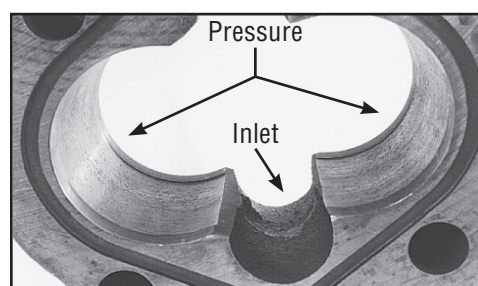
This pump housing shows a deep gearpath (.014") caused by overpressurization. Acceptable cutout must measure .005" or less to provide satisfactory service. High pressure forces the pump gears to the inlet or low pressure side of pump. When excessive pressure occurs, the gears deflect causing abnormal gear cutout.
