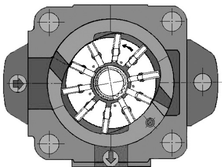
Cross section of vane pump
