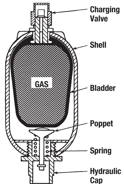
The Bladder Accumulator
