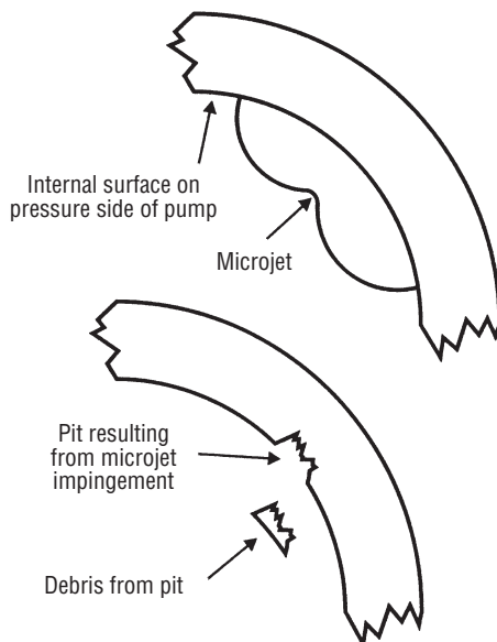
Pitting results from the collapse of air or gas bubbles on the internal surface of the pump.
