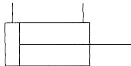
Cylinder, double acting
