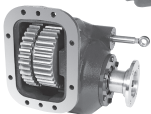
Power Take-Offs used to transfer engine power to a hydraulic pump.
