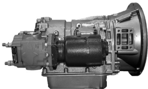
Muncie CS Series PTO and PK1 Series gear pump mounted to an Allison® automatic transmission.
